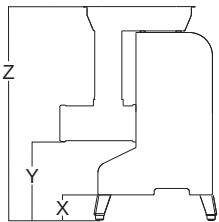
Gambe basse con piedino Short legs with feet X: 131 mm Y: 271 mm Z: 741 mm
